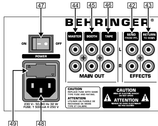
Fig. 3.2: PRO MIXER DJX700 rear panel connectors
