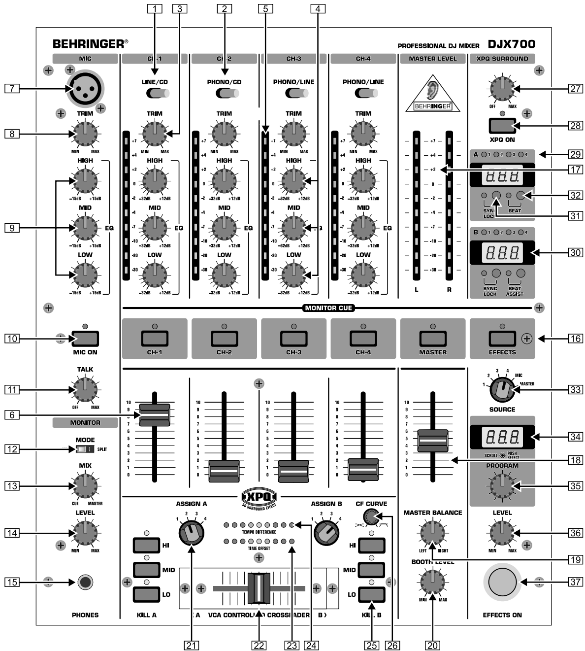
Fig. 2.1: PRO MIXER DJX700 control elements
