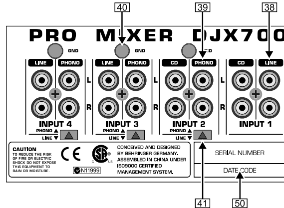
Fig. 3.1: PRO MIXER DJX700 rear panel connectors
